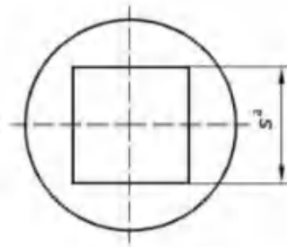
Figure C.3—Gauge for verifying form tolerance specified in Figures 24 and 72
