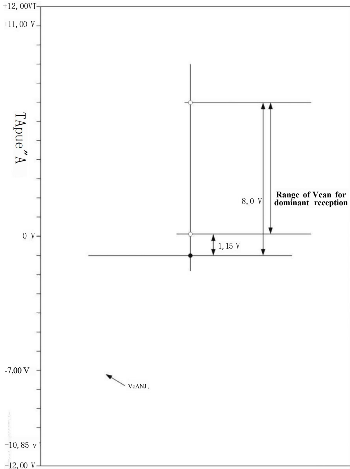
Figure A.4—Valid voltage range of V_{CAN\_H} for monitoring dominant state while the HS-PMA is not connected to the media, when V_{CAN\_L} varies from minimum to maximum common mode range during low-power mode
